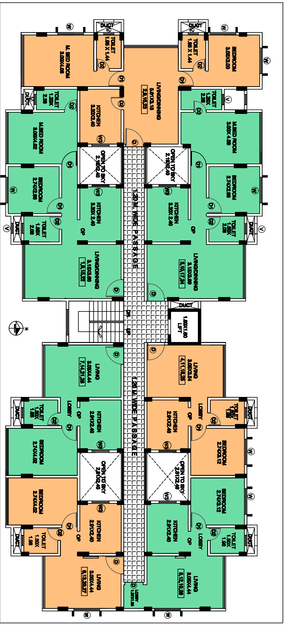
TYPICAL FLOOR PLAN FOR STILT, 1ST, 2ND & 3RD FLOORS
